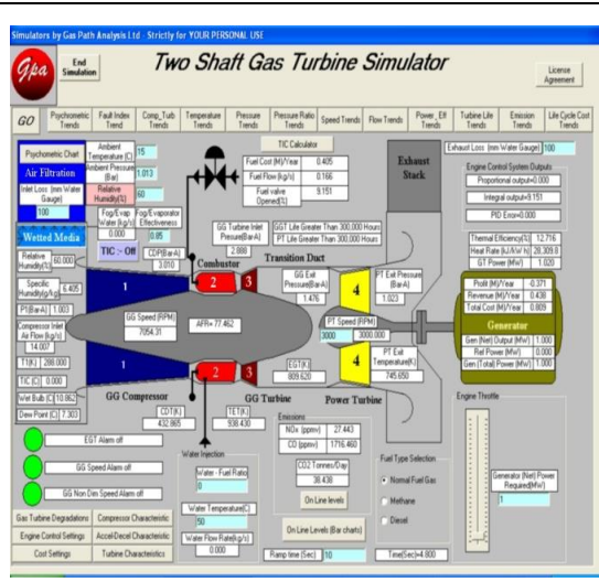
Two Shaft Gas Turbine Simulator
